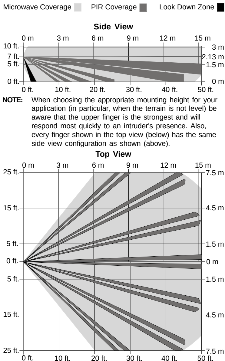
Figure 1 - Coverage Patterns
