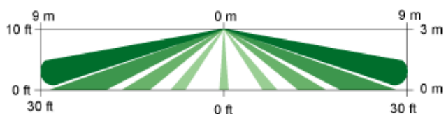
AR8-13 Side View
