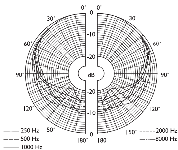
Polar diagram (measured with pink noise)
