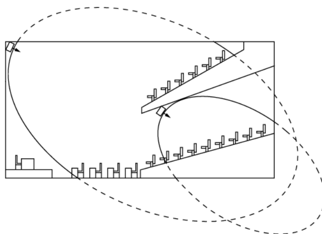
Figure 17: Radiators covering seats beneath a balcony
