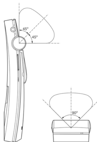
Figure 4: Directional characteristics of the receivers
