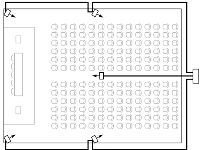
Figure 25: Symmetrical radiator cabling (recommended)
