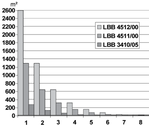
Figure 5: Total coverage area of LBB 4511/00, LBB 4512/00 and LBB 3410/05 for 1 to 8 carriers
