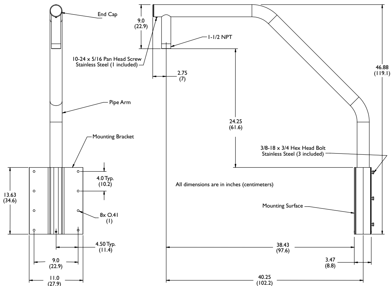
Figure 3. Dimensions LTC 9230/00 Parapet Mount
