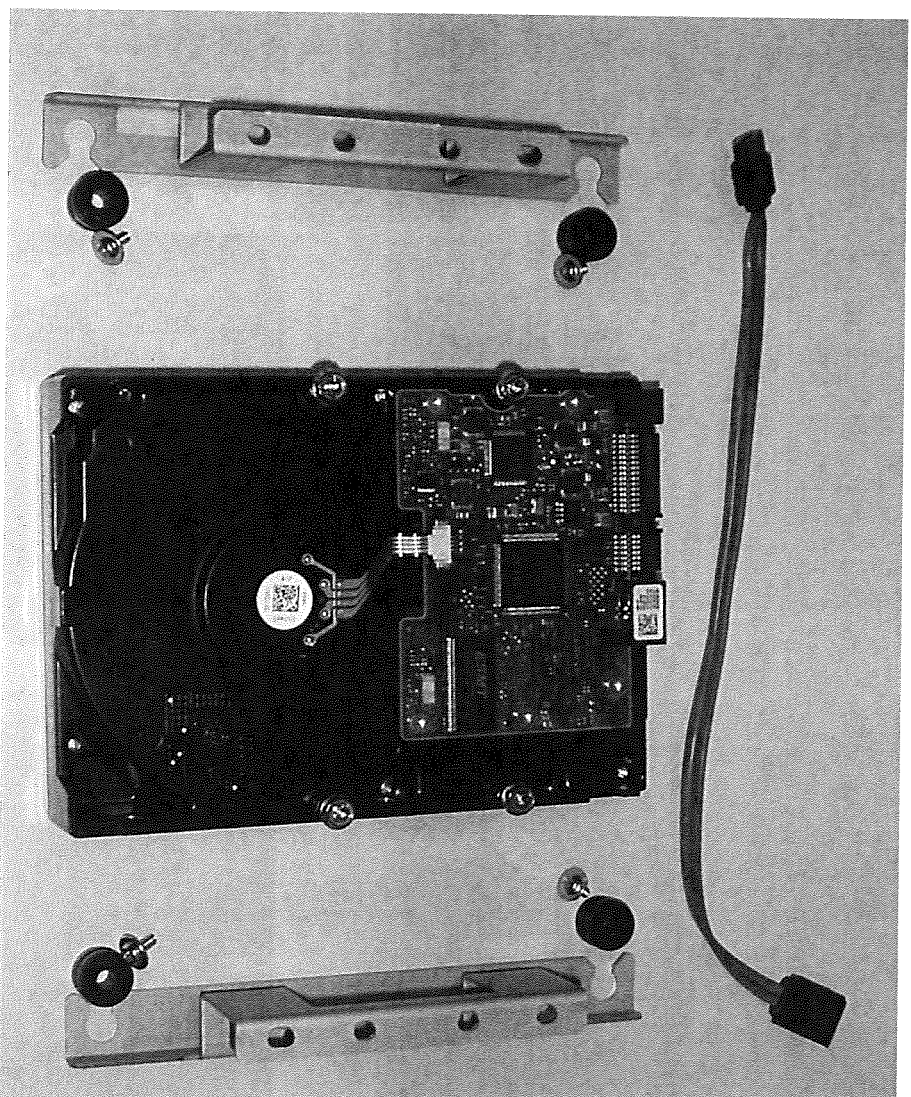
Figure 5.4: Install HDD 1 (DIVAR 3000)
