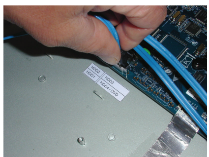
Figure 11.10: Install DVD in DIVAR AN 5000
