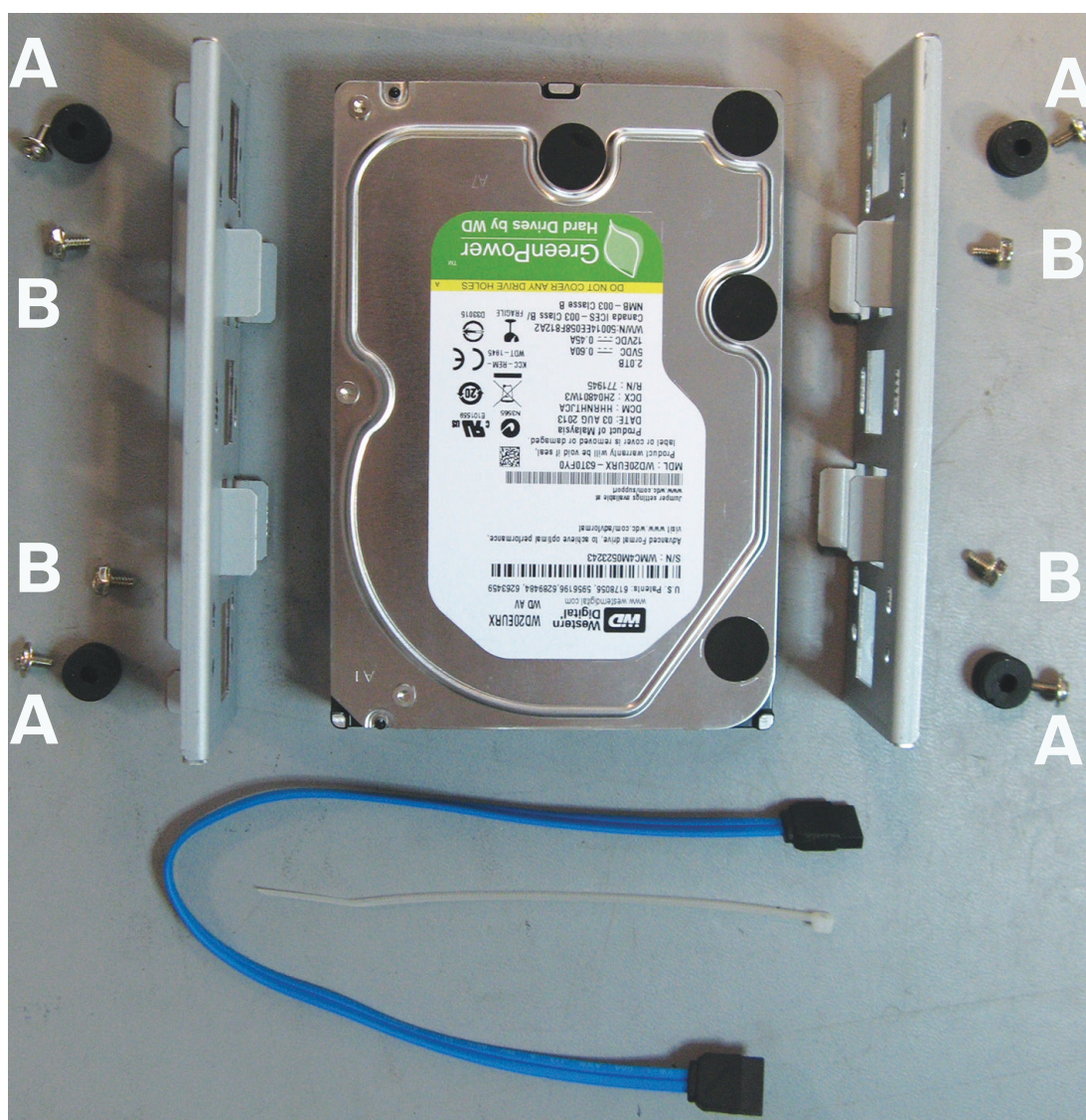
Figure 11.6: HDD install components for DIVAR AN 5000
