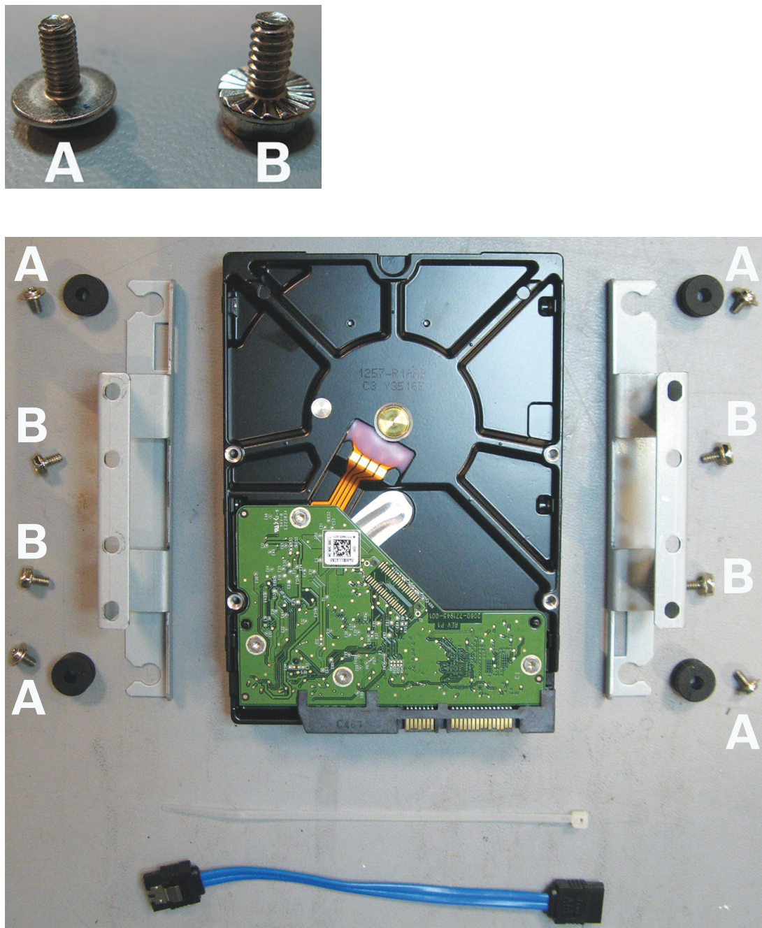
Figure 11.4: HDD install components for DIVAR AN 3000
