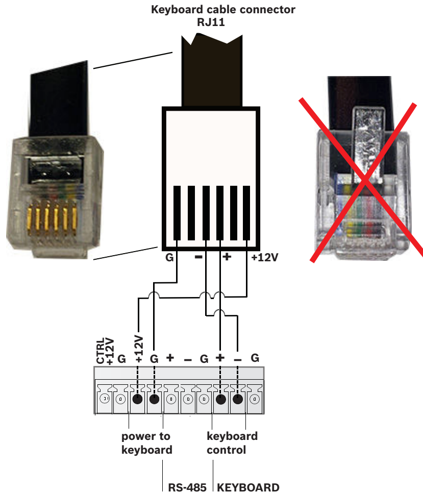
Figure 5.2: RJ11 adaptor connections
