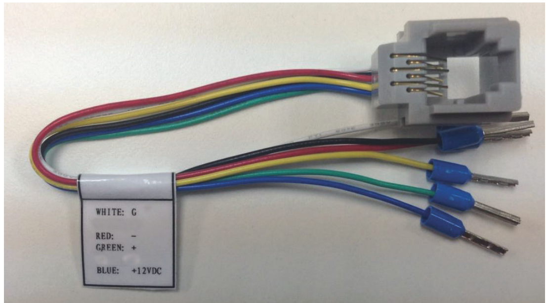
Figure 5.1: RJ11 adaptor
