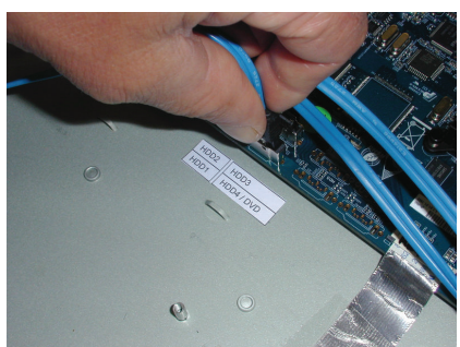
Figure 11.14: Install DVD in DIVAR 5000
