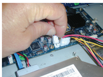
Figure 11.12: Install DVD in DIVAR 3000
