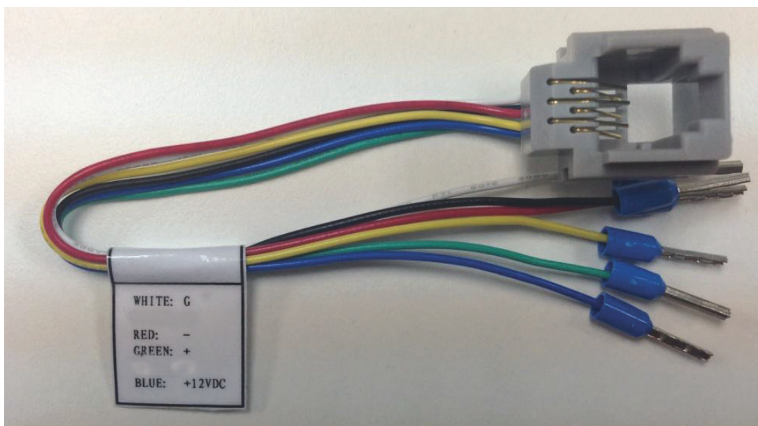
Figure 5.1: RJ11 adaptor
