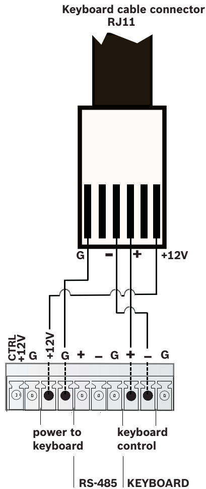
Figure 5.2: Keyboard connector
