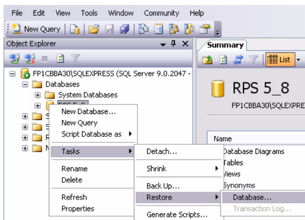
Figure 5.10 SQL Server 2005
