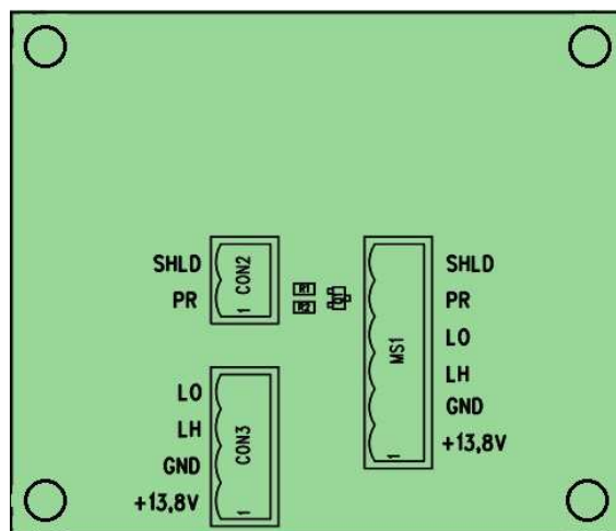
Figure 13 Topographical arrangement of the components in the circuit
