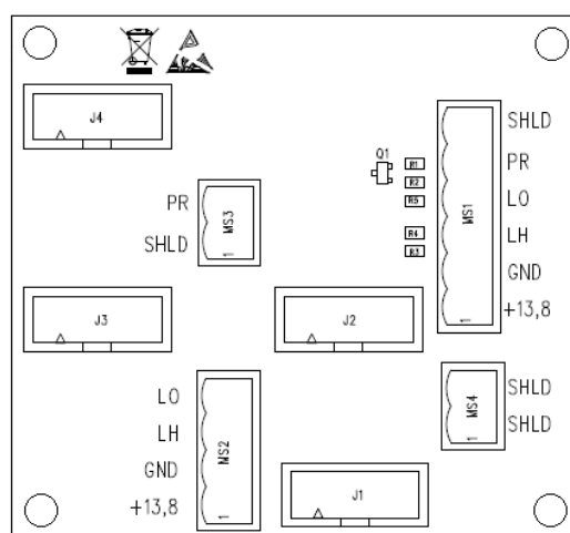
Figure 13 Topographical arrangement of the components in the circuit
