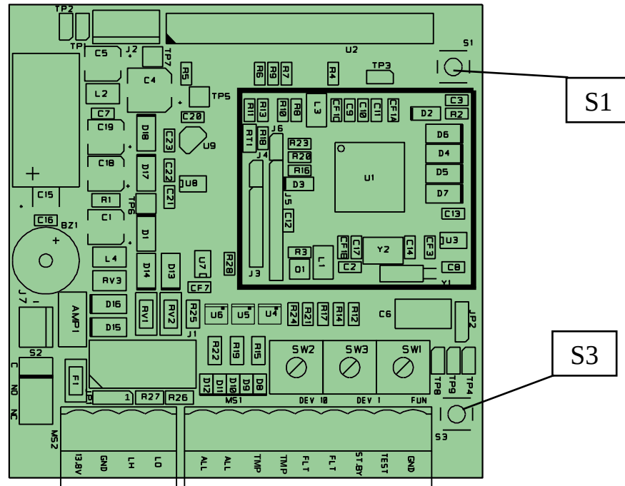
Figure 12 Topographic arrangement of the components in the circuit
