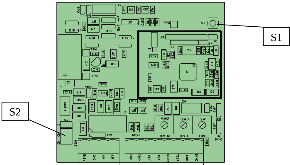
Figure 11 Topographical arrangement of the components in the circuit
