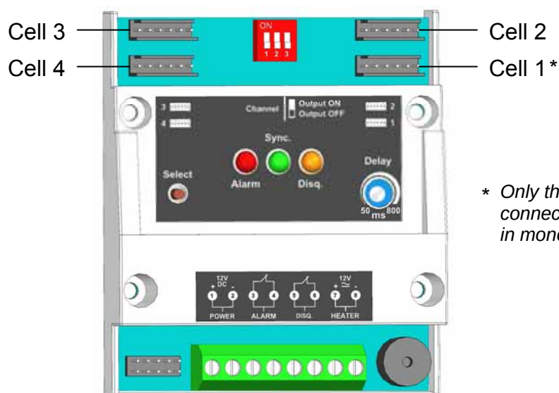
Cell cabling
