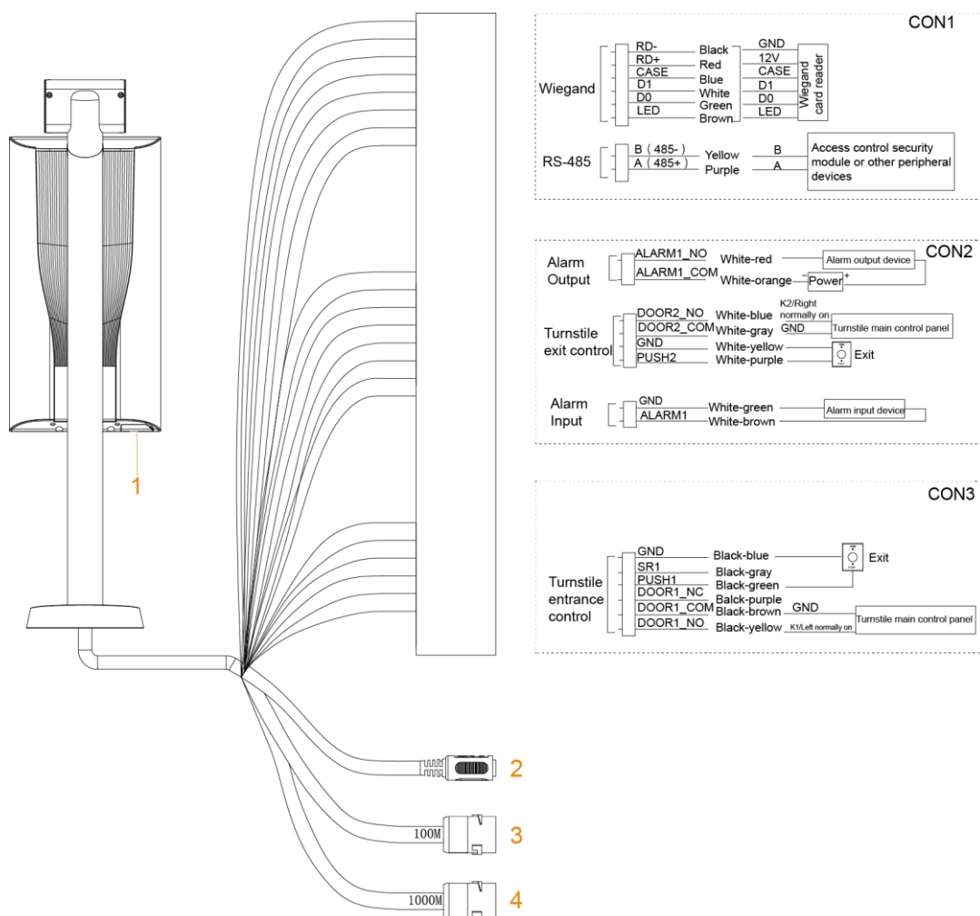
Figure 2-1 Collegamento Cavi
