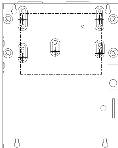
SP5500 (8x10")
