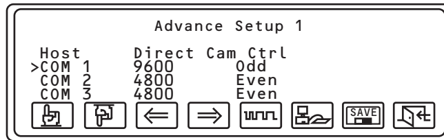
Figure 15. Baud and Parity
