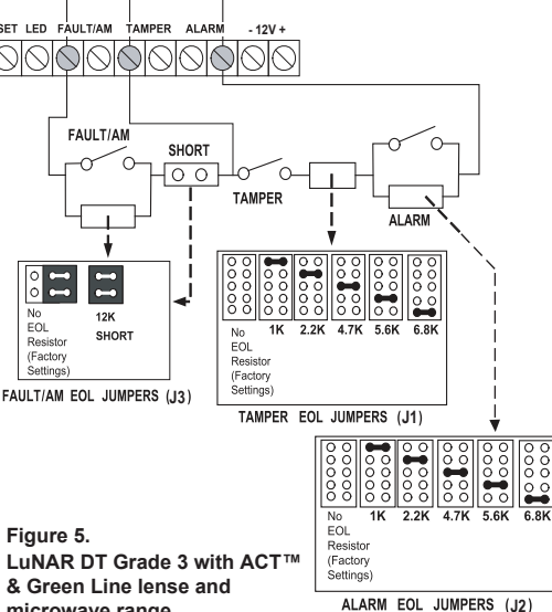
Figure 5. LuNAR DT Grade 3 with ACT™ & Green Line lense and microwave range
