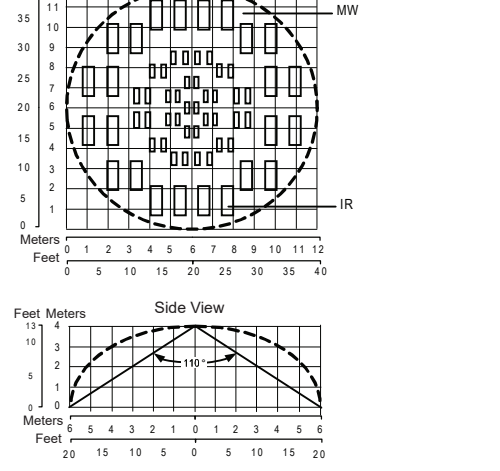
Figure 5. LuNAR DT Grade 3 with ACT™ & Green Line lense and microwave range
