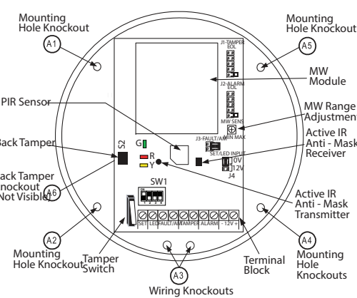
Figure 3. Terminal Wiring
