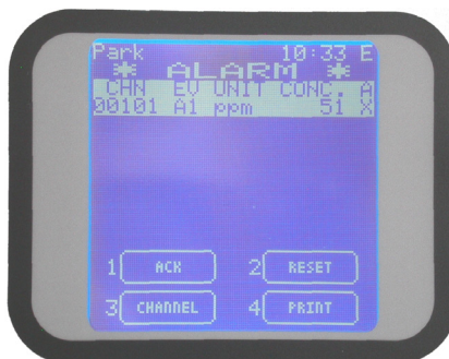
Figure 27) Active Events screen with alarm only
