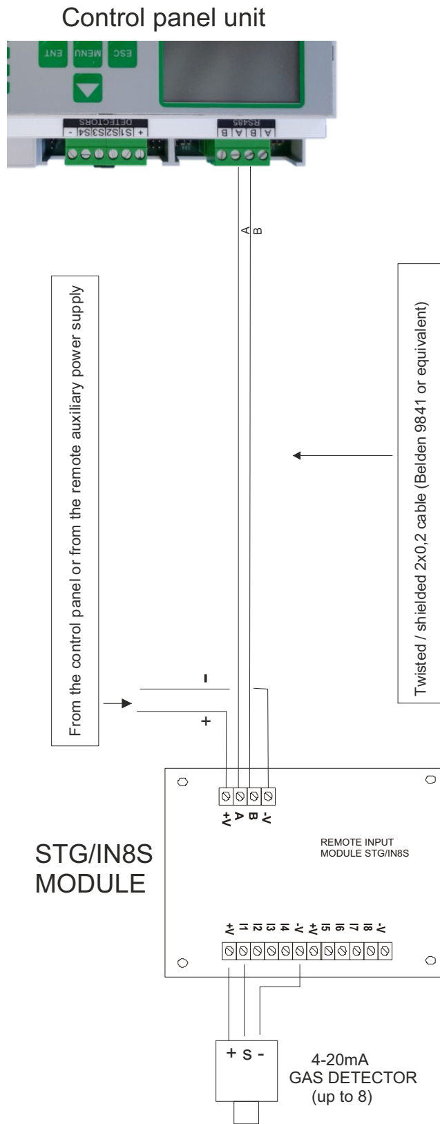
Figure 13) Detector connection by STG/IN8S
