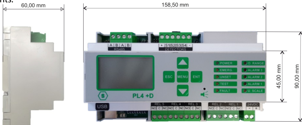
Figure 1) Global dimensions PL4 +D
