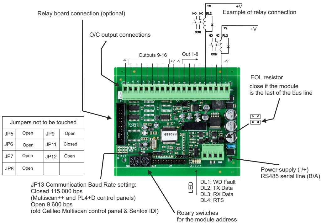
Figure 15) STG/OUT16S module
