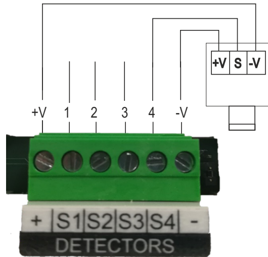
Figure 10) Connection of the 4 detectors of the gas control unit
