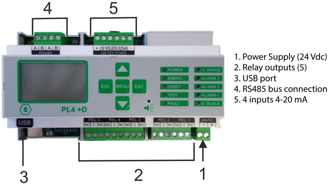
Figure 5) Part identification
